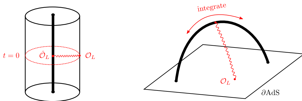
Figure 1: Comparison of our approach and the approach of [3, 4]. Left: In our approach, we use a radial-quantization picture and compute a matrix element of a light operator \mathcal{O}_L between two D-brane states. This translates to a matrix element of a dual operator \hat{\mathcal{O}}_L defined on the D-brane worldvolume. Right: The approach of [3, 4]. They considered a trajectory of a D-brane emitted and absorbed from the AdS boundary. They then attached a supergravity mode to the D-brane and integrated over its position.
