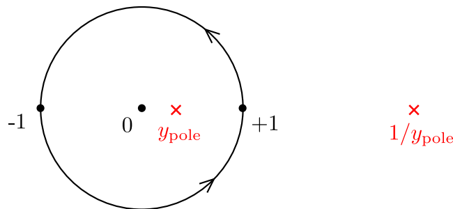
Figure 2: Positions of poles of the y -integral in (3.59). The integrand has two poles: for s \ll 1 , one of them is inside the integration contour while the other is outside.
