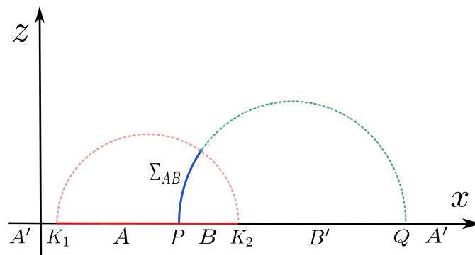
Figure 3: The x coordinates for points K_1, P, K_2 and Q are a, p, b, q . The PEE is given by s_{AA'}(A) = s_{BB'}(B) which is dual to the EWCS \Sigma_{AB} (shown by the blue line).
